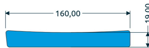
DETAIL B | BOTTOM LOGO SCALE 1:3
